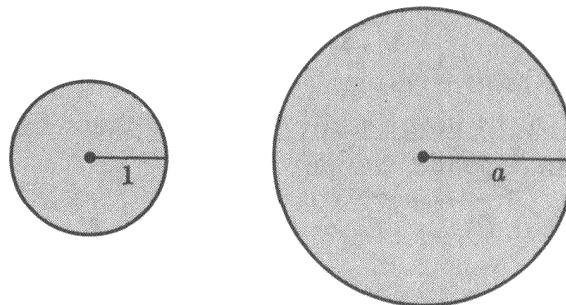
Disc of radius 1
