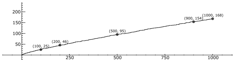
FIGURE 1.1. Graph of \pi(x) for x < 1000
