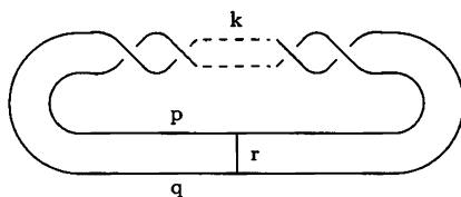
FIGURE 13.5. Orbifold G_k(p, q; r) .
