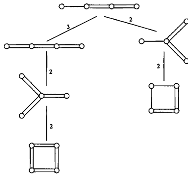
FIGURE 13.3. Coxeter symbols for non-compact hyperbolic tetrahedra whose groups are commensurable with \text{PSL}(2, O_1) . The diagram shows the commensurability relationships, the figures giving the indices of the groups.
