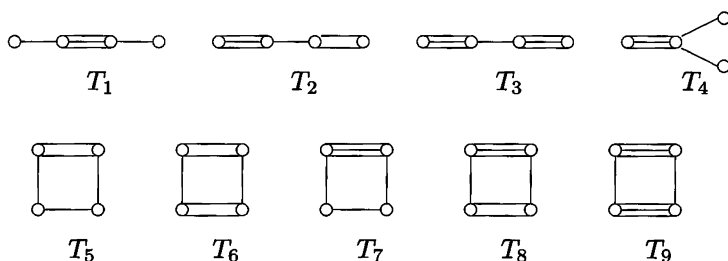
FIGURE 13.1. Coxeter symbols for compact hyperbolic tetrahedra.
