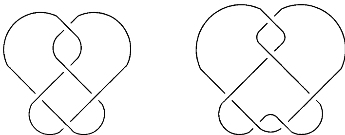
FIGURE 4.3. The knots 5_2 and 6_1 .
