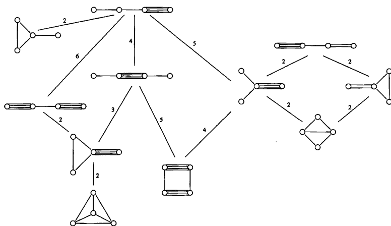
FIGURE 13.2. Coxeter symbols for non-compact hyperbolic tetrahedra whose groups are commensurable with \mathrm{PSL}(2, \mathcal{O}_3) . The diagram shows the commensurability relationships, the figures giving the indices of the groups.
