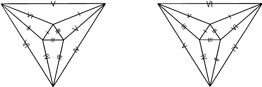
FIGURE 4.2. Identification scheme for Borromean Rings complement
