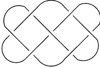
FIGURE 4.1. Knot 7_4 .
