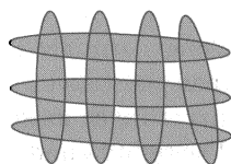
not pseudodisks
