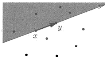
a 4-facet
