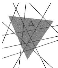
I(\Delta)
