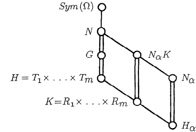
FIGURE 4.1. Subgroup lattice
